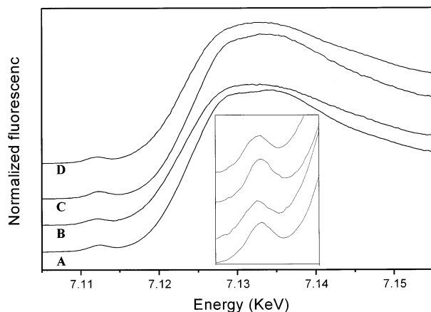
Fig. 1. Edge spectra of native (A) and substrate complexed (B) HQ1,2O from Nocardioideis simplex and of native (C) and substrate complexed (D) ClC1,2O from Rhodococcus erythropolis (ClC1,2O) samples. In the inset are shown enlargements of the pre-edge peak regions.
